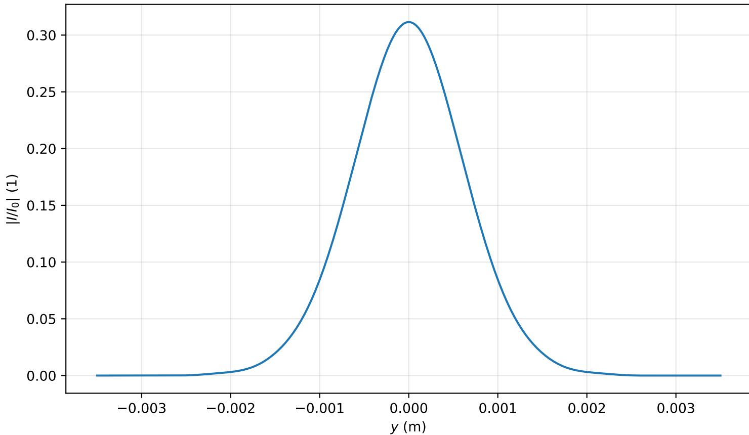
Intensity profile I(x = 0, y, z = 3.742)/I_0 , P_{in}=0.3P_{cr} , artificial time
